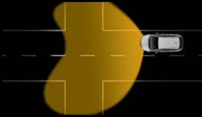
Pedestrian Area Light (up to 30 km/h). Highlights potential hazards with a wider spread of light (an extra 8° left and right).
